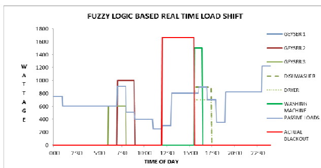
Fig. 6 Fuzzy Logic Based Real Time Optimized Individual Load Curve
