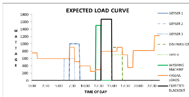
Fig. 4 Expected Individual Load Schedule
