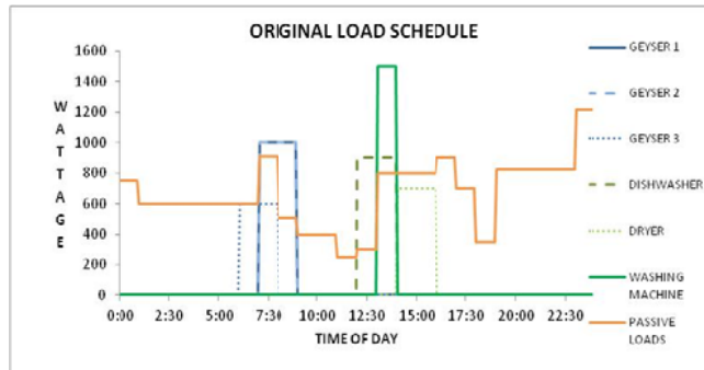
Fig. 2 Individual Load Schedule
