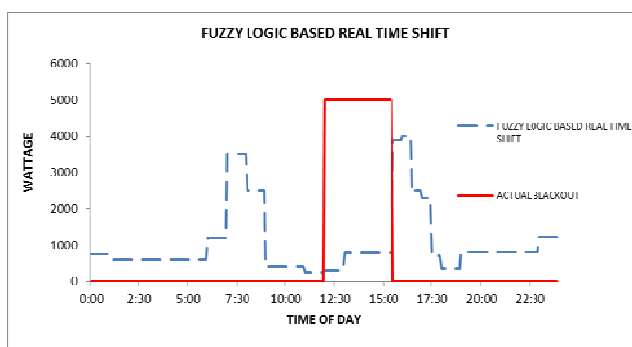
Fig. 5 Fuzzy Logic Based Real Time Optimized Load Curve
