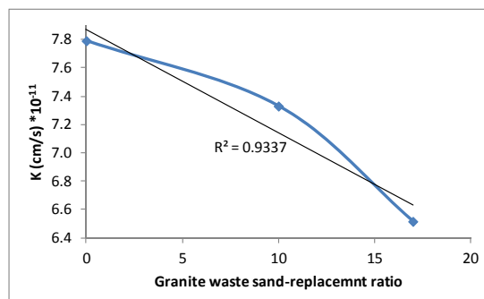
Fig. 6b. Permeability coefficient for sand replacement waste ratios
