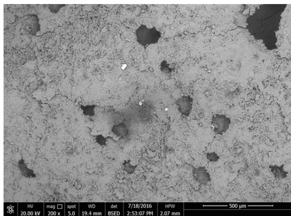
Fig. 8a. SEM image of control mix (CM) at 200X
