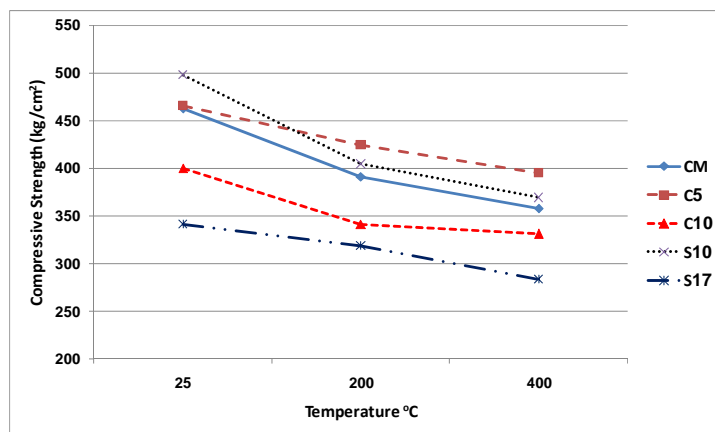
Fig. 5. Relation between temperature and compressive strength
