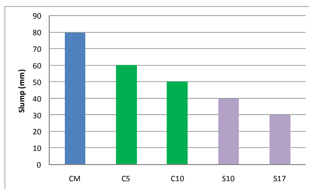
Fig. 4. Slump test results
