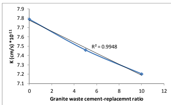
Fig. 6a. Permeability coefficient for cement replacement waste ratios
