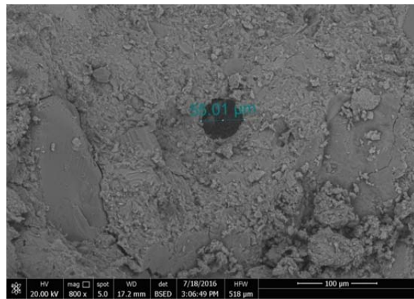
Fig. 9b. SEM image of 5% cement replacement (C5) at 800X
