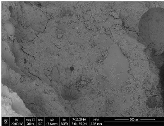
Fig. 9a. SEM image of 5% cement replacement (C5) at 200X
