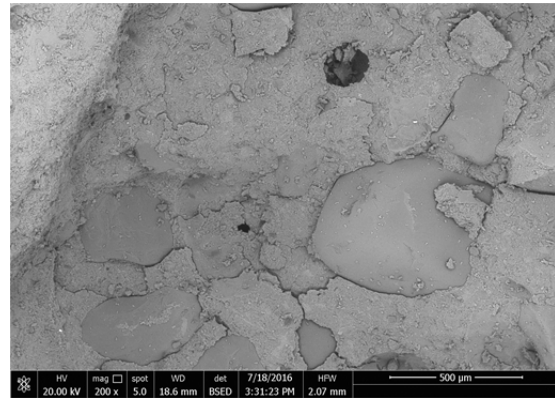
Fig. 12. SEM image of 17% sand replacement (S17) at 200X
