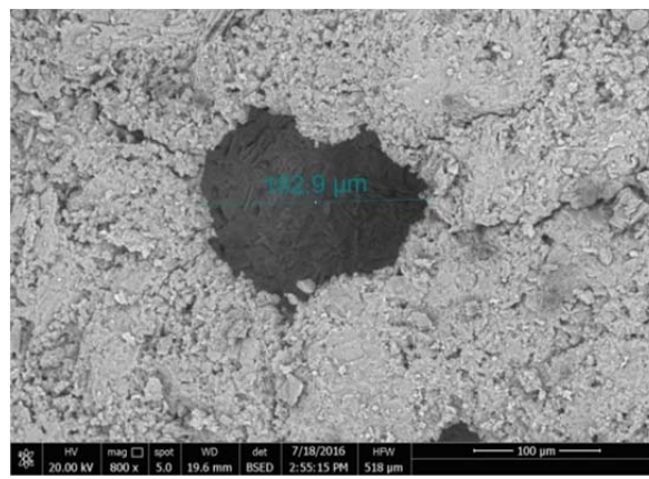
Fig. 8b. SEM image of control mix (CM) at 800X
