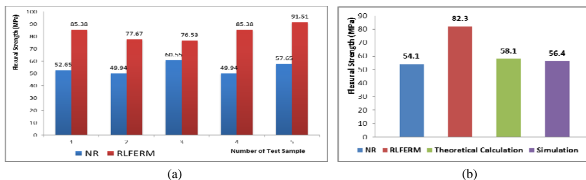
Fig. 6. Flexural strength of NR and RLFERM
