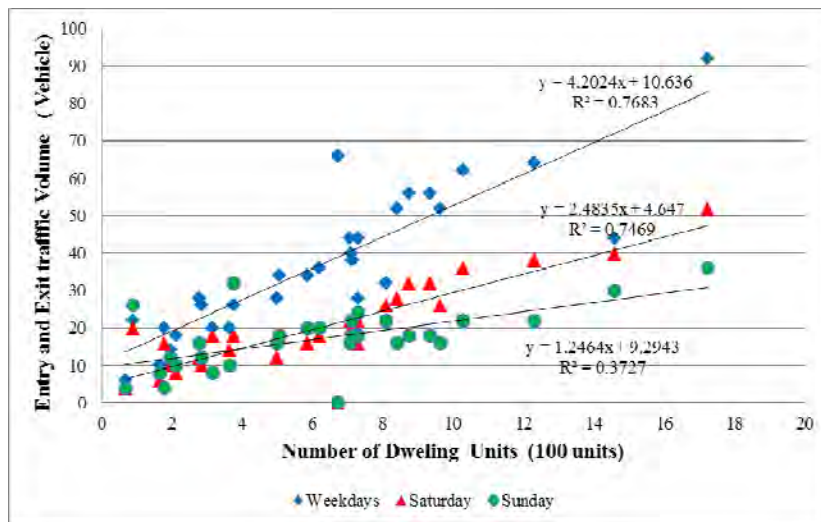
Fig. 3. All vehicle types; entry and exit volume versus dwelling units
