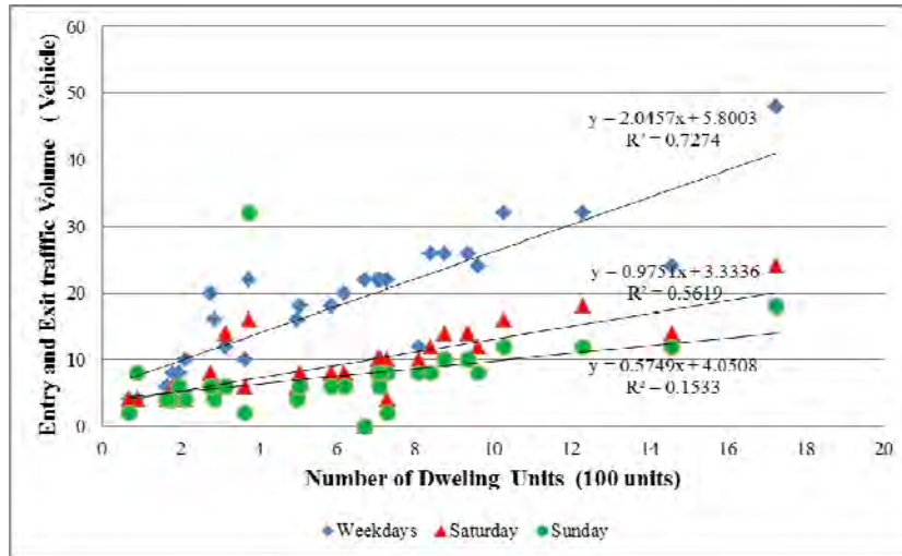
Fig. 4. Six-wheeled and ten-wheeled trucks; entry and exit volume versus dwelling units
