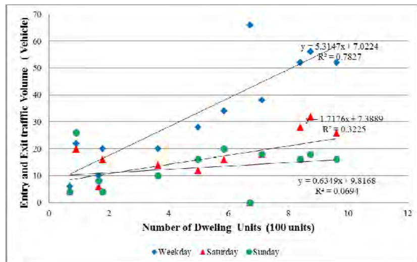
Fig.6. Entry and exit volume versus dwelling units of low rise condominium projects
