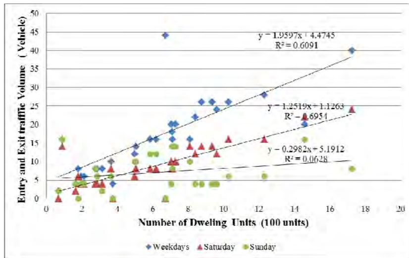
Fig. 5. Four-wheeled trucks and passenger cars; entry and exit volume versus dwelling units
