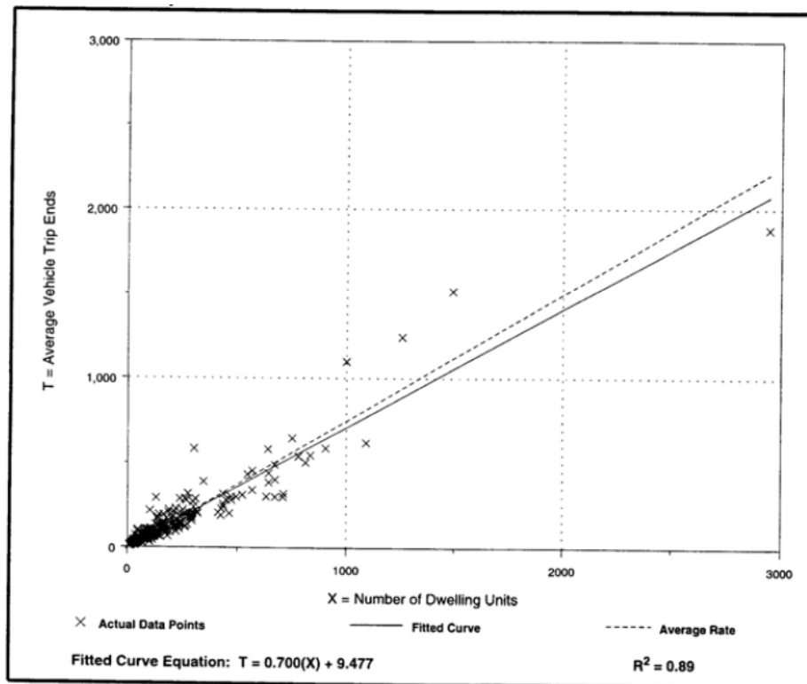
Fig. 1. Example of ITE trip generation rates and equation [2]
