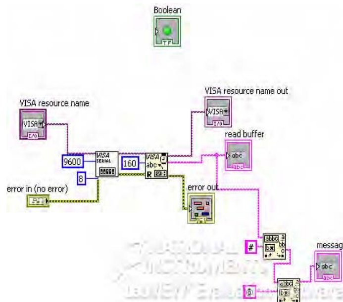
Fig.12. ZIGBEE Reception
