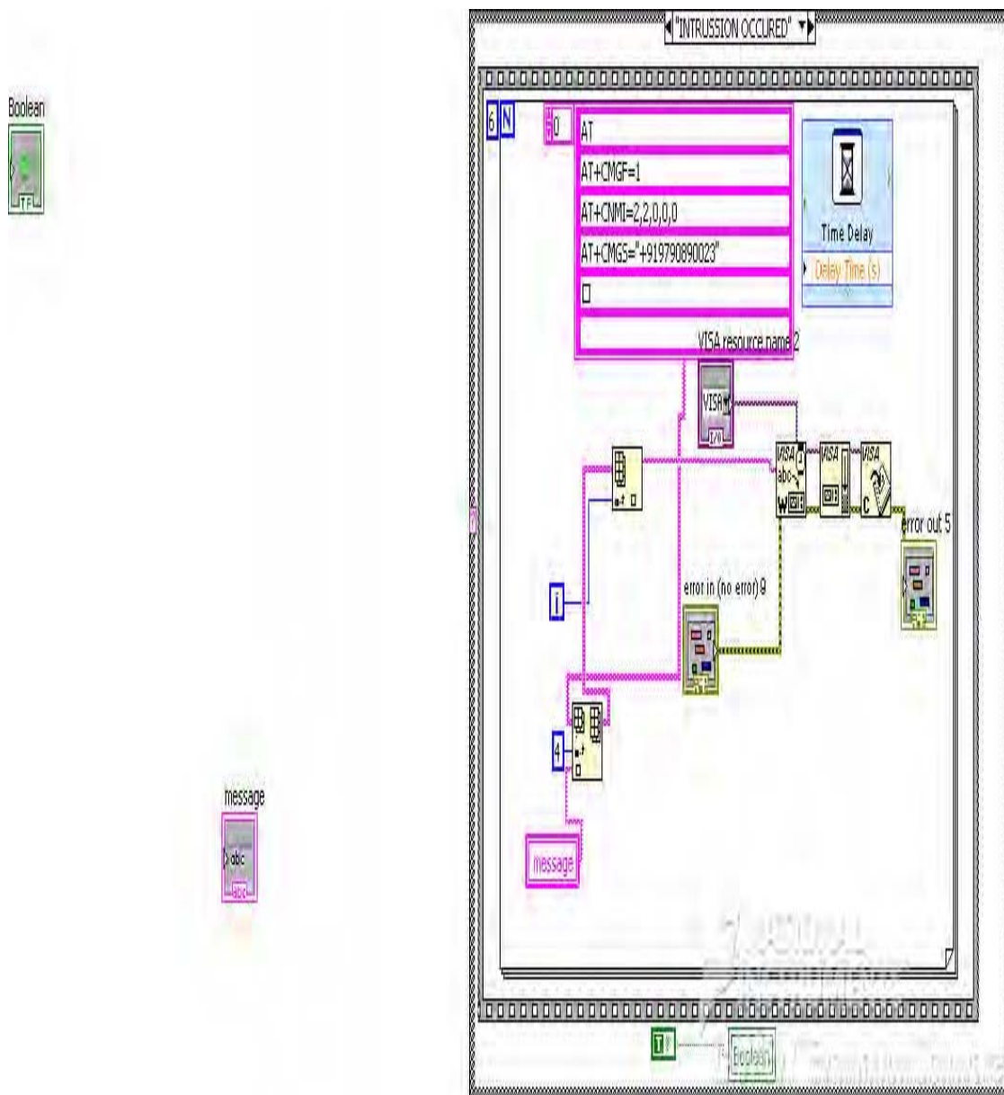
Fig.14. GSM Transmission
