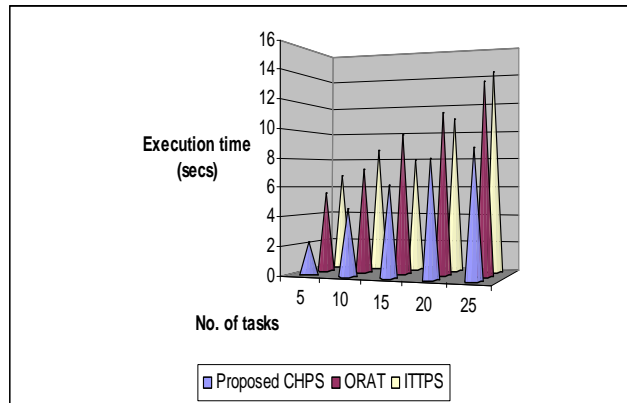
Fig.3: No. of tasks Vs. Execution time
