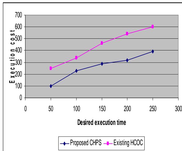
Fig.6: Execution time vs. Execution cost
