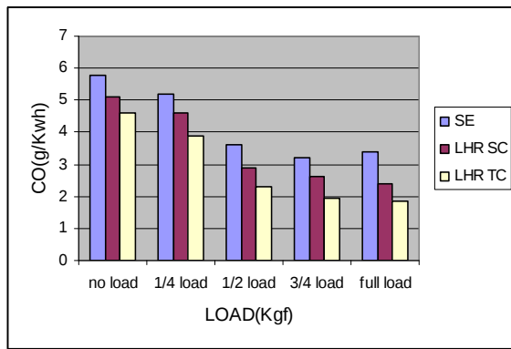
Fig.4 Load Vs CO emission
