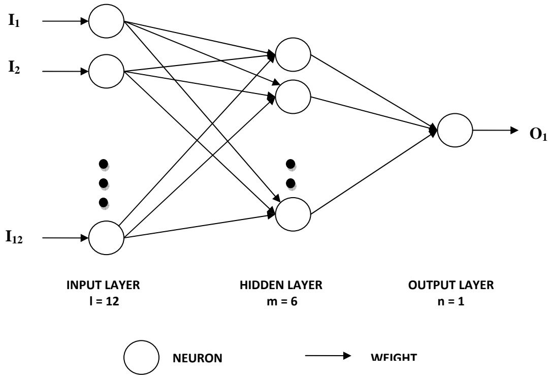
Figure 4: Neural Network Architecture for Fruit Grading Model
