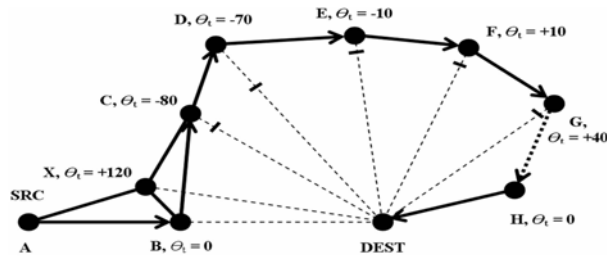
Fig.1 Greedy-Bounded Compass Routing
