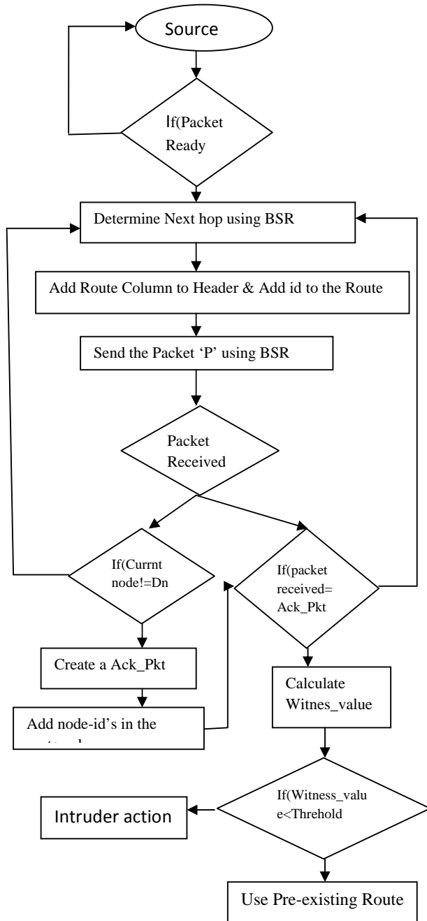
Fig.4 Flowchart for RRS scheme
