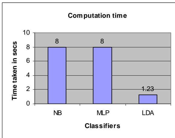
Fig. 5 Computation Time
