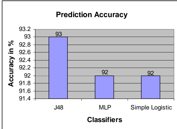
Fig. 4 Prediction Accuracy
