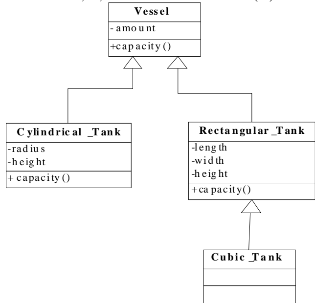
Figure 3. Static class diagram for case study I
